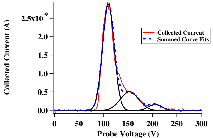
Figure 5. ExB Ion Current Integration Method
