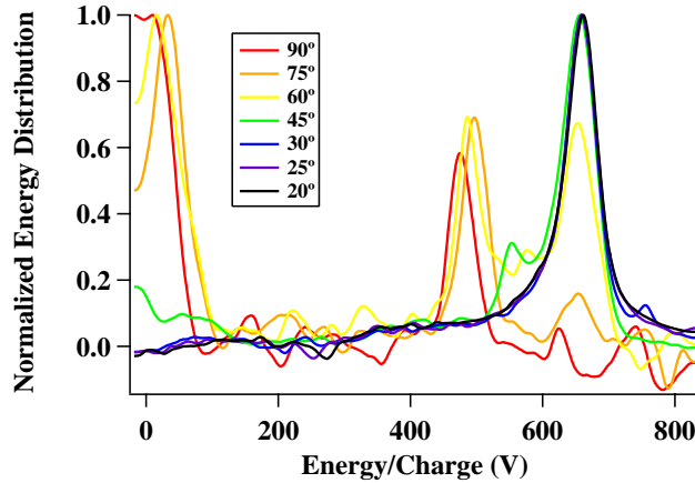
Figure 6. Normalized Voltage Distribution Function for Operation Point 12
