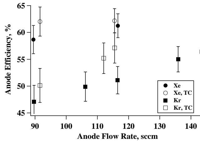
Figure 9. Anode Efficiency versus Anode Flow Rate
