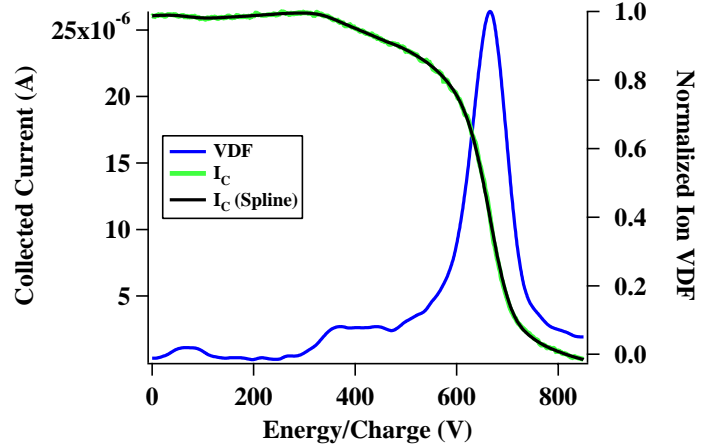
Figure 4. Retarding Potential Analyzer Data Processing Example
