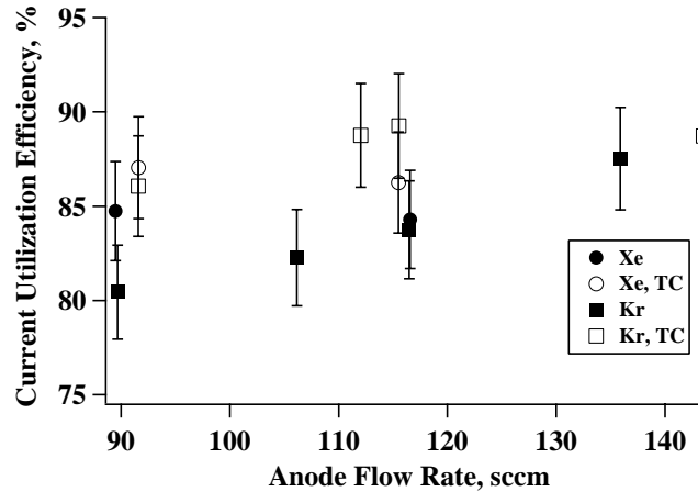
Figure 11. Current Utilization Efficiency versus Anode Flow Rate
