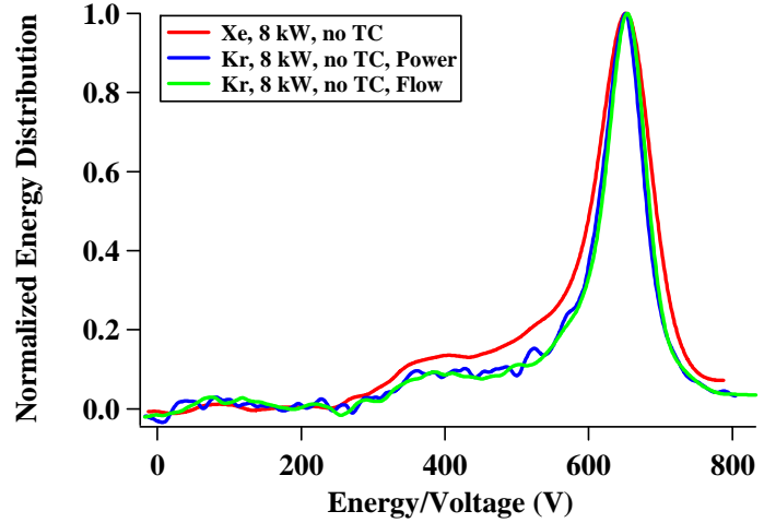
Figure 7. Voltage Energy Distribution Comparison for Xenon and Krypton at 8 kW without the Trim Coil
