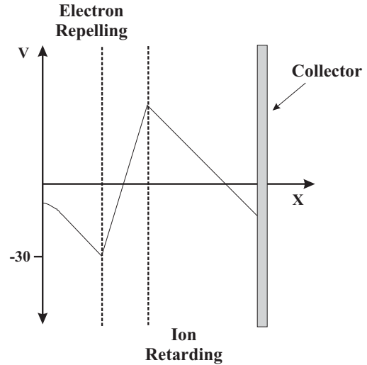
Figure 3. Retarding Potential Analyzed Potential Diagram
