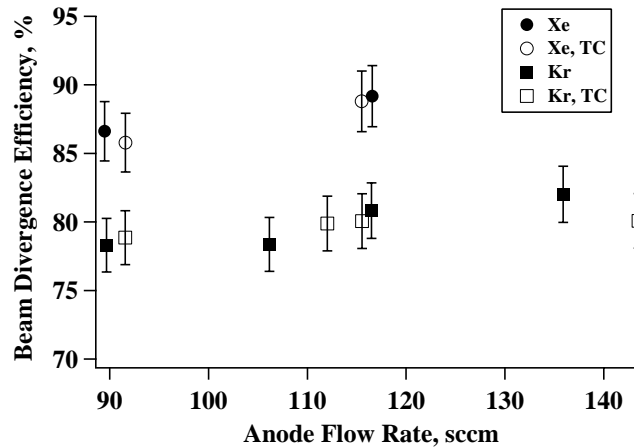
Figure 12. Beam Divergence Efficiency versus Anode Flow Rate
