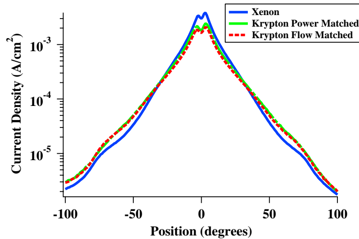
Figure 8. Ion Current Density Comparison of the 8 kW Case without the Trim Coil
