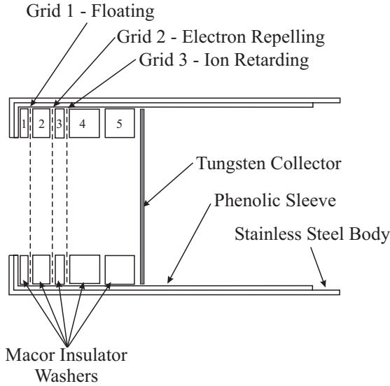
Figure 2. Retarding Potential Analyzer Schematic
