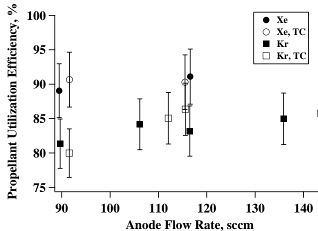
Figure 10. Propellant Utilization Efficiency versus Anode Flow Rate
