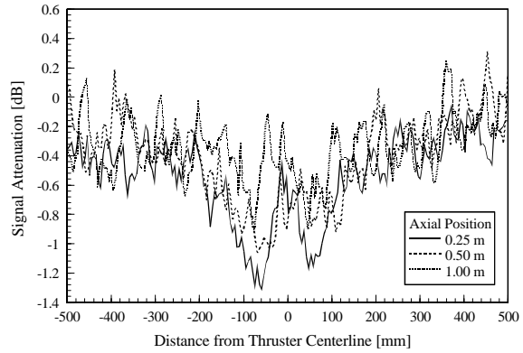
Figure 11: Signal Attenuation for 300 V Discharge Voltage
