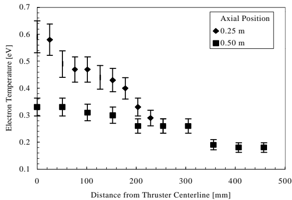
Figure B1: Electron Temperature for 300 V Discharge Voltage
