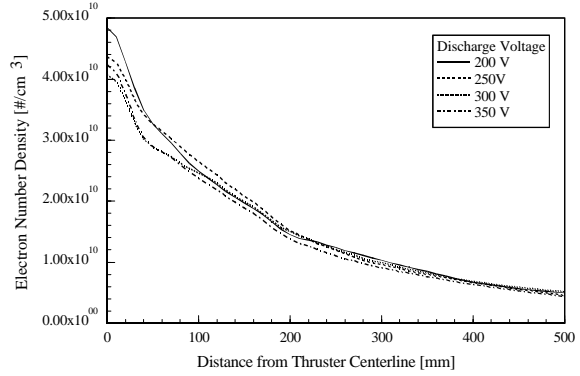
Figure 13: Electron Number Density at 0.50 m Axially
