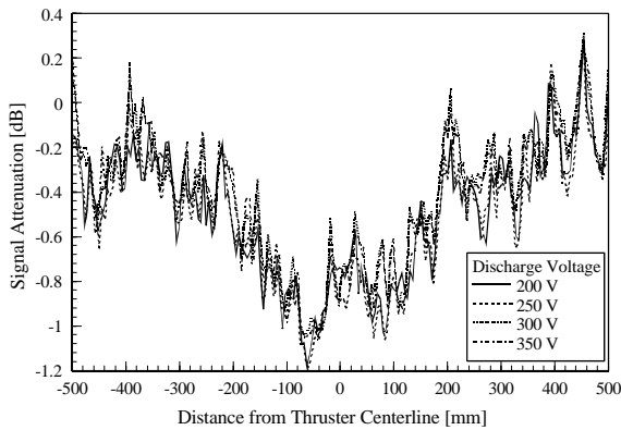
Figure 9: Signal Attenuation at 0.50 m Axially
