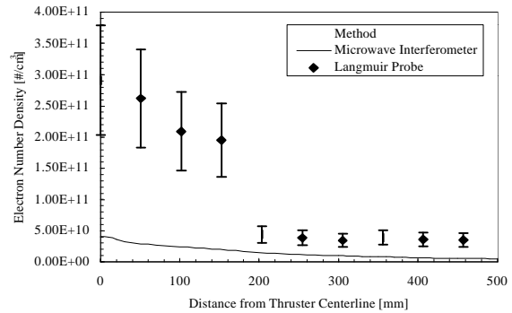
Figure B3: Comparison of Electron Density Results at 0.50 m Axially
