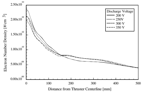
Figure 14: Electron Number Density at 1.00 m Axially
