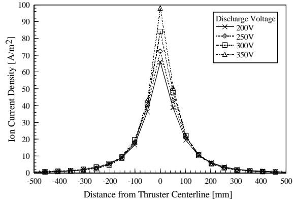
Figure A2: Ion Current Density at 0.50 m Axially
