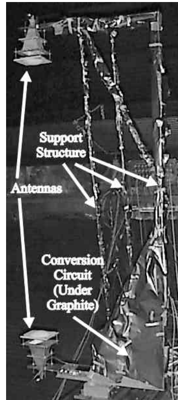
Figure 2: Microwave Interferometer
