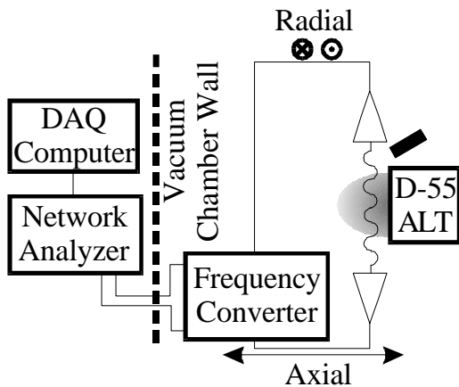
Figure 1: Experimental Setup
