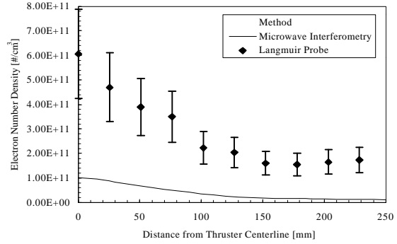
Figure B2: Comparison of Electron Density Results at 0.25 m Axially
