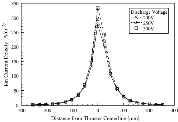
Figure A1: Ion Current Density at 0.25 m Axially
