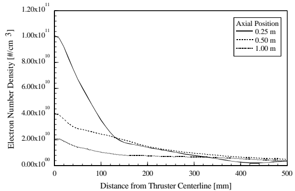
Figure 15: Electron Number Density for 300 V Discharge Voltage
