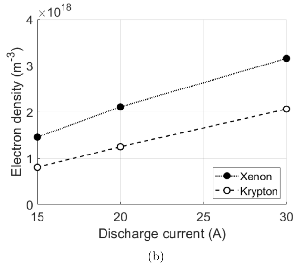
Figure 14. Average plasma density in channel of xenon and krypton operation for (a) increasing discharge voltage with a constant discharge current of 15 A, and (b) increasing discharge current with a constant discharge voltage of 300 V.
