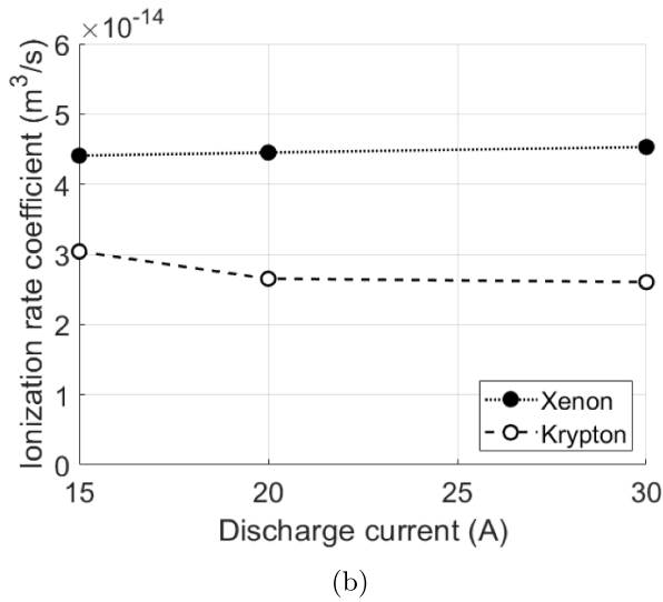
Figure 13. Average ionization rate coefficient in channel of xenon and krypton operation for (a) increasing discharge voltage with a constant discharge current of 15 A, and (b) increasing discharge current with a constant discharge voltage of 300 V.
