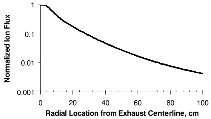
Figure 2. A representative radial profile of the ion flux in the Hall thruster plume, 93 cm downstream from the exit plane of the thruster, with Hall thruster parameters of 150 V, and 16.6 A, 15 mg/s Xe.
