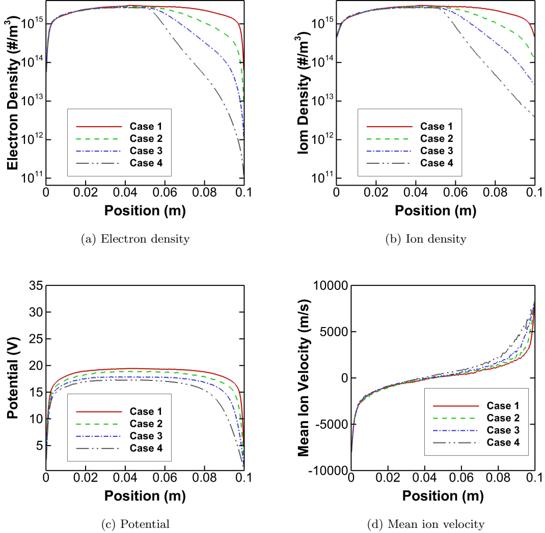
Figure 7: Set 1, density effect simulations.
