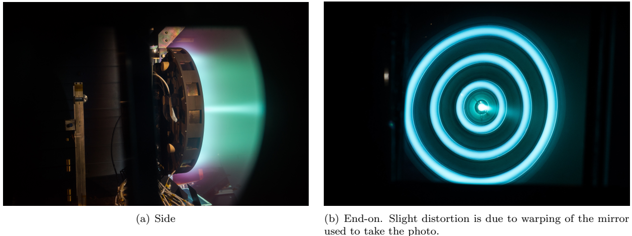
Figure 1. Photographs from two angles of the X3 firing at 50 kW total discharge power in VF5 at NASA GRC.
