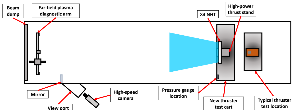
Figure 3. A schematic showing the location of the X3 as well as diagnostic equipment inside VF5. Schematic is not to scale.
